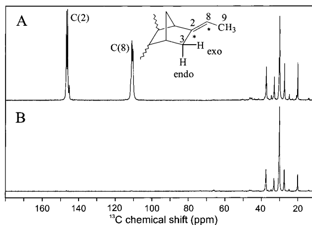
Figure 3. ^1\text{H} -decoupled ^{13}\text{C} MAS NMR spectra of labeled (A) and unlabeled EPDM (B).
